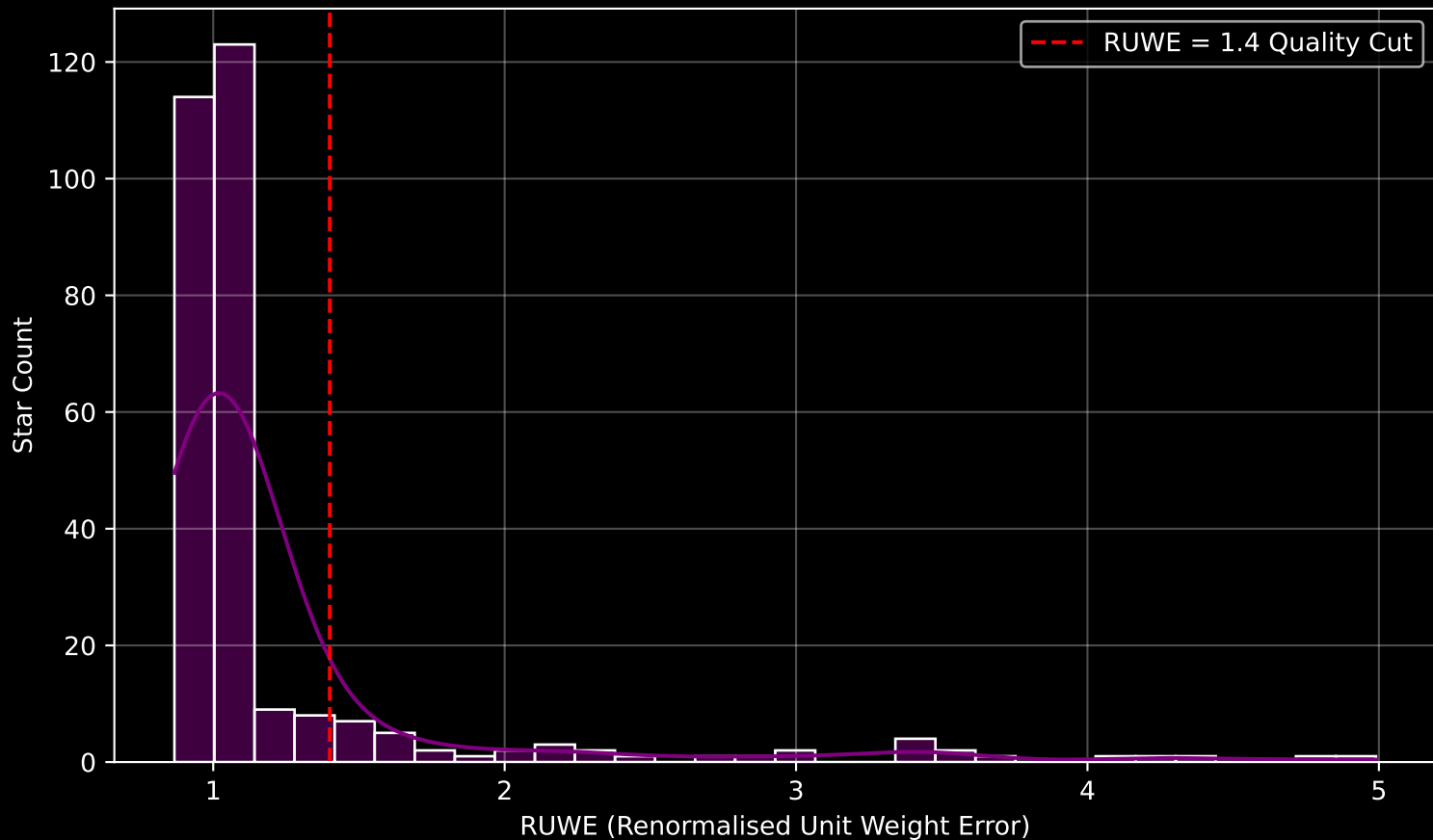
GALAH DR4 Field [557] RUWE Distribution (n= 293)
