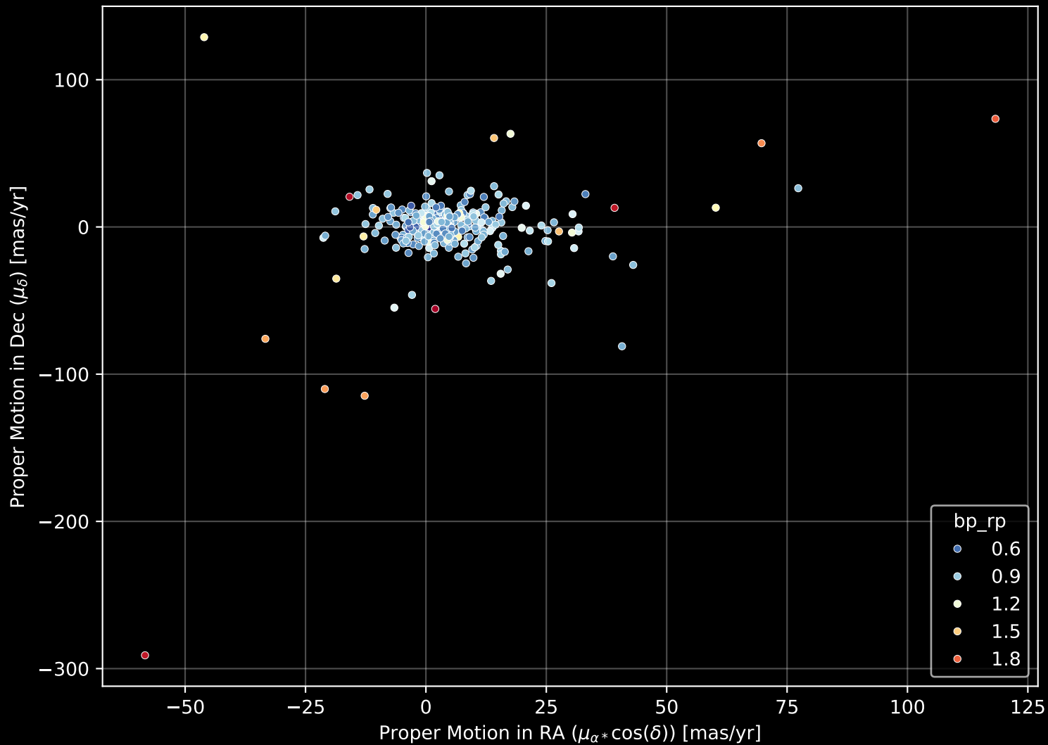
GALAH DR4 Field: [557] Proper Motion Diagram (n= 306)
