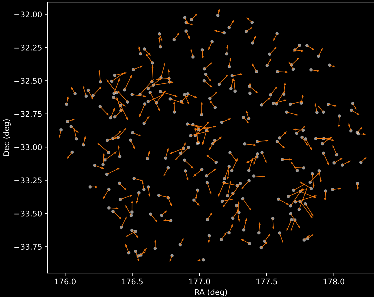
GALAH DR4 Cluster 2 Proper Motion Vectors (n=244)
