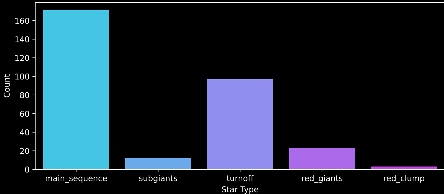
GALAH DR4 Field: [557] Count plot of Star Type
